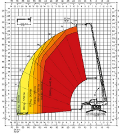
REP 2-4,5 Nacelle extensible rotative 500 kg
