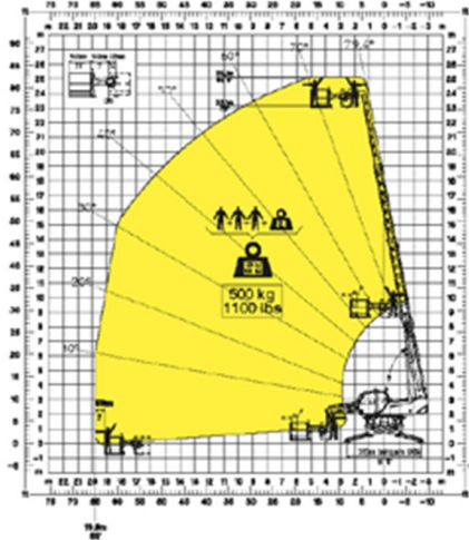
REP 2.2 Nacelle rotative non extensible 500 kg
