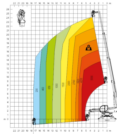
J 600 potence 600 KG
